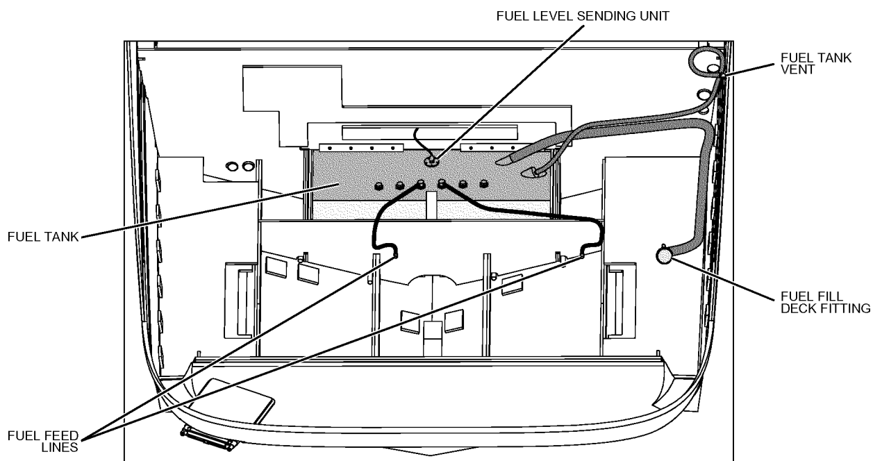
GAS ENGINE FUEL LINE ROUTING (IF EQUIPPED)
