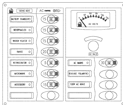
110-VOLT AC MASTER PANEL (IF EQUIPPED WITH DUAL SHORE POWER)
